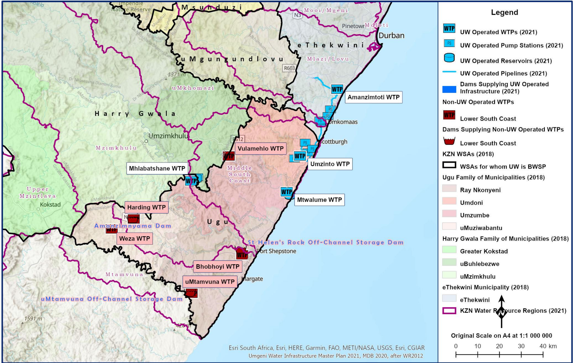
Figure 11.1 General layout of the South Coast System.
