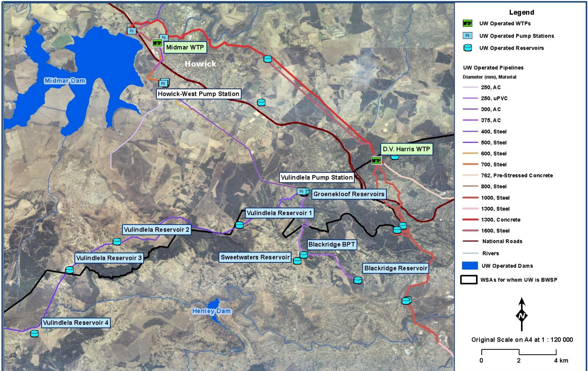
Figure 7.31 General Layout of the Howick-West Sub-System.
