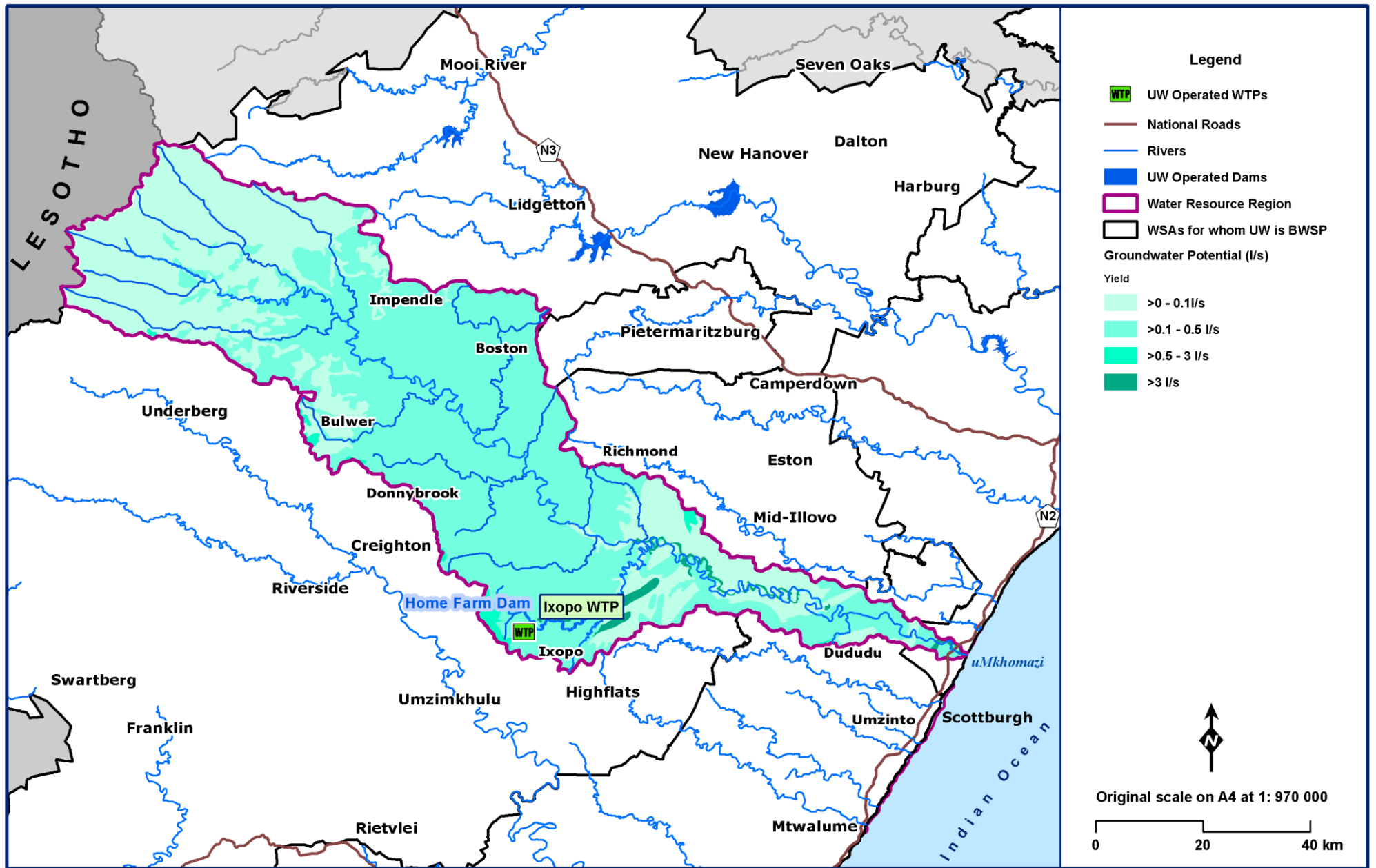
Figure 7.19 Groundwater potential in the Mkhomazi Region (KZN DoT 2011; MDB 2016; Umgeni Water 2017; WR2012).
