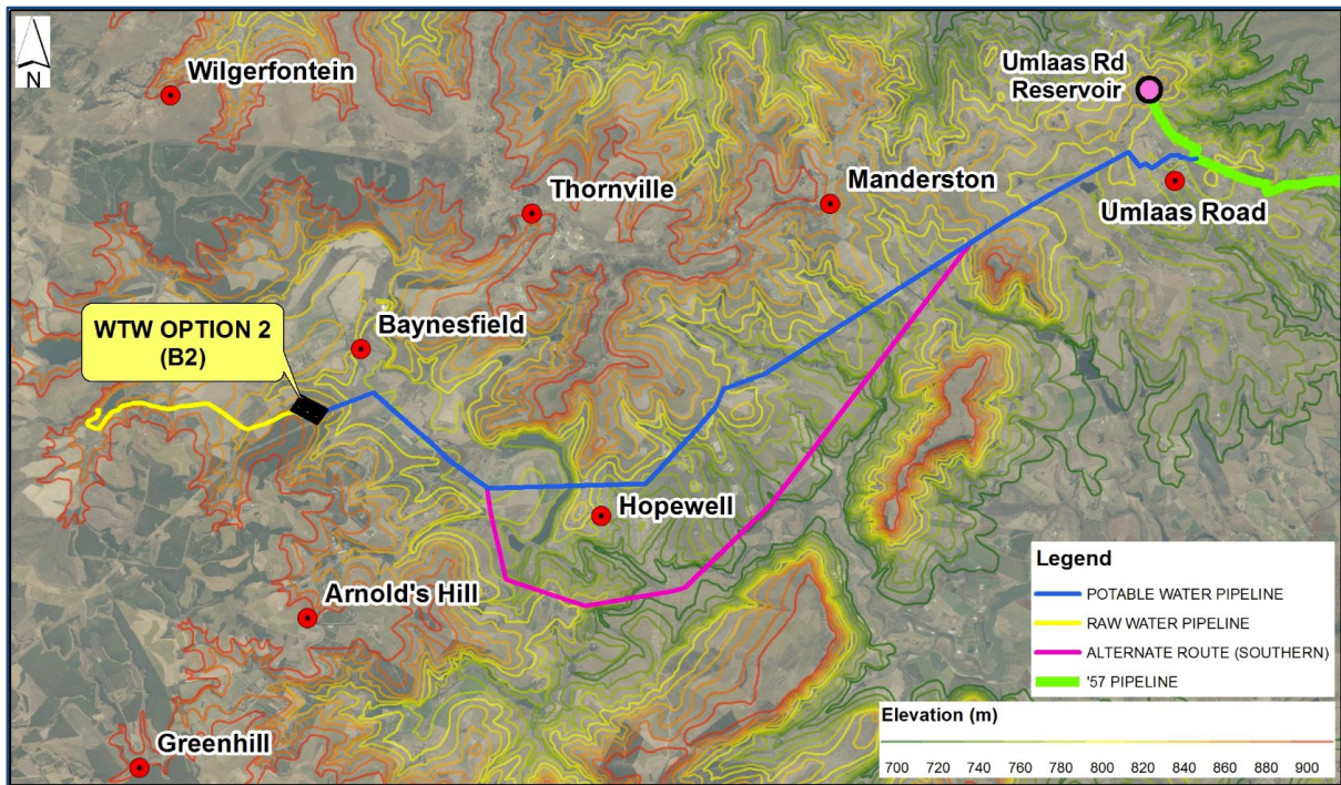
Figure 7.62 Layout of pipeline.
