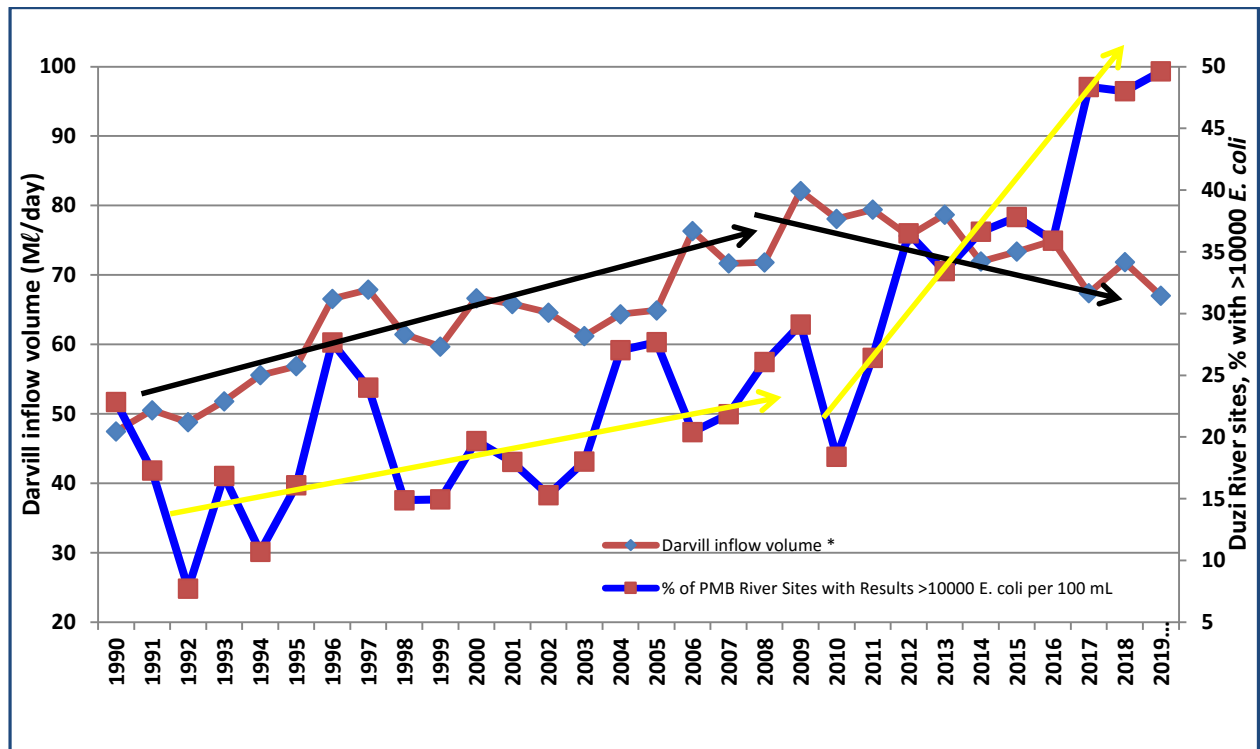
Figure 7.15 Darvill WWW Annual Median Inflow Volume and Msunduzi River Sites with E. coli Numbers >10 000 per 100ℓ.
