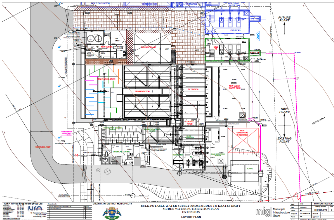
Figure 7.95 General layout of the Muden WTP upgrade.
