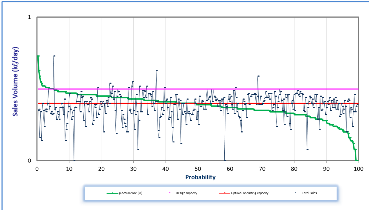
Figure 7.76 Analysis of historical production at Applesbosch WTP (November 2018 to October 2019).
