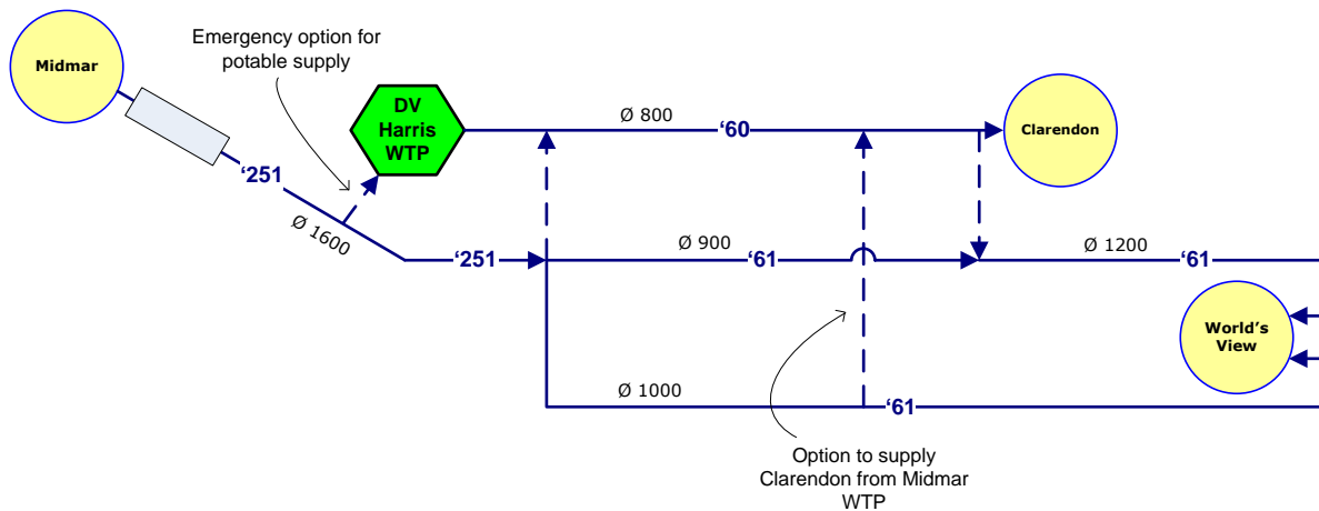
Figure 7.33 Pipeline configuration between D.V. Harris WTP and World's View Reservoir.
