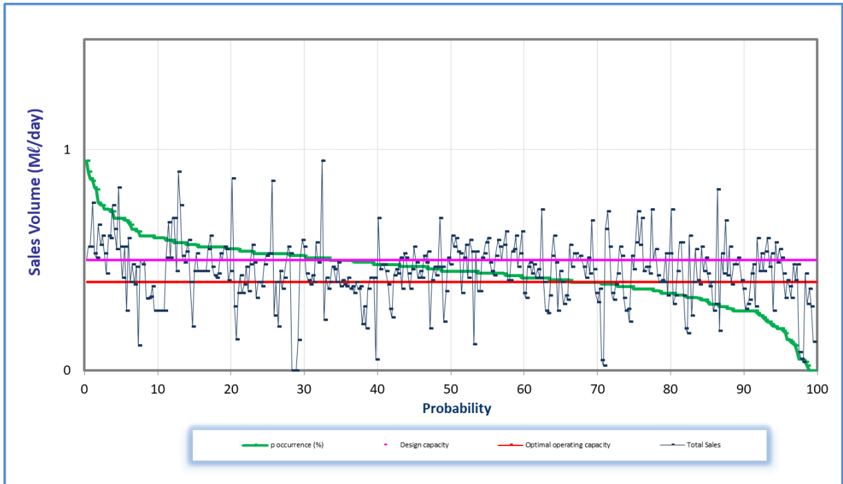
Figure 7.81 Analysis of historical production at Lidgett WTP (November 2018 to October 2019).
