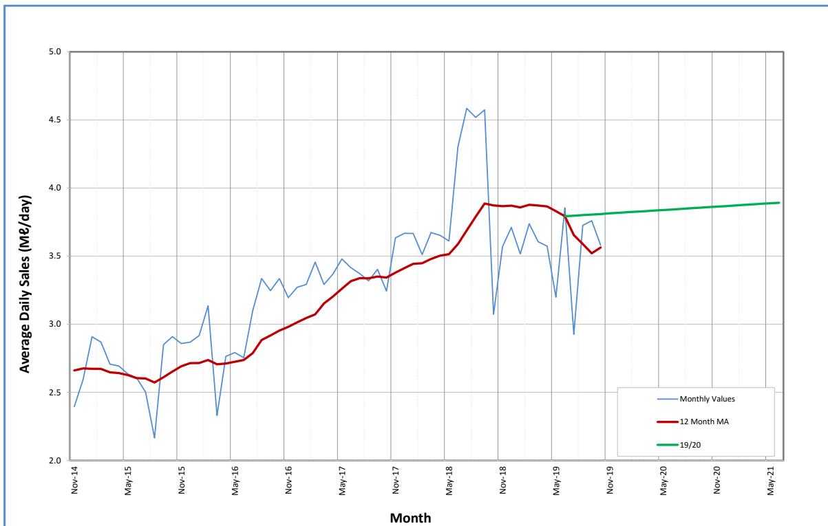
Figure 7.50 Historical demand curve and projections for Maphephethwa WTP.
