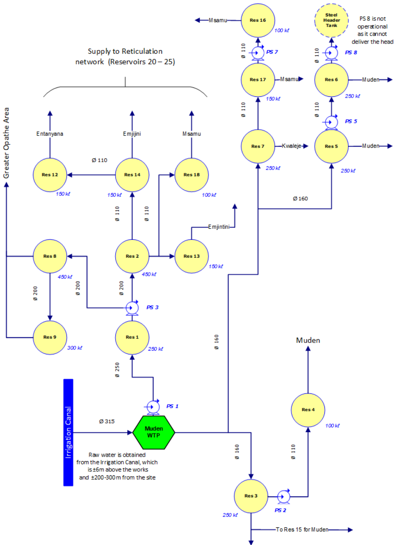
Figure 7.93 Schematic of the Mudén Supply System.
