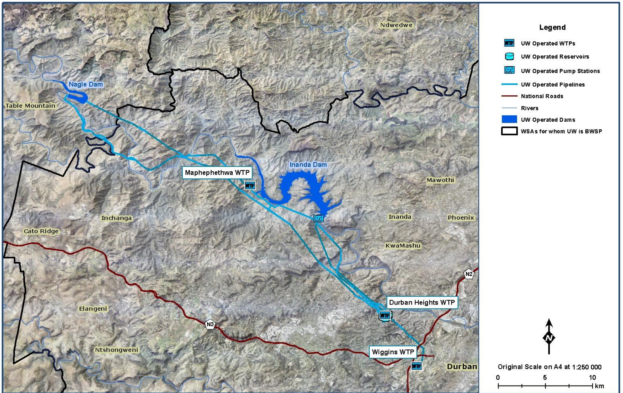
Figure 7.5 General layout of the Lower Mgeni System.
