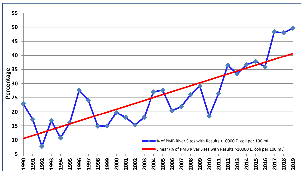
Figure 7.14 Percentage of Msunduzi catchment river sites with E. coli results > 10000 per 100 ml.
