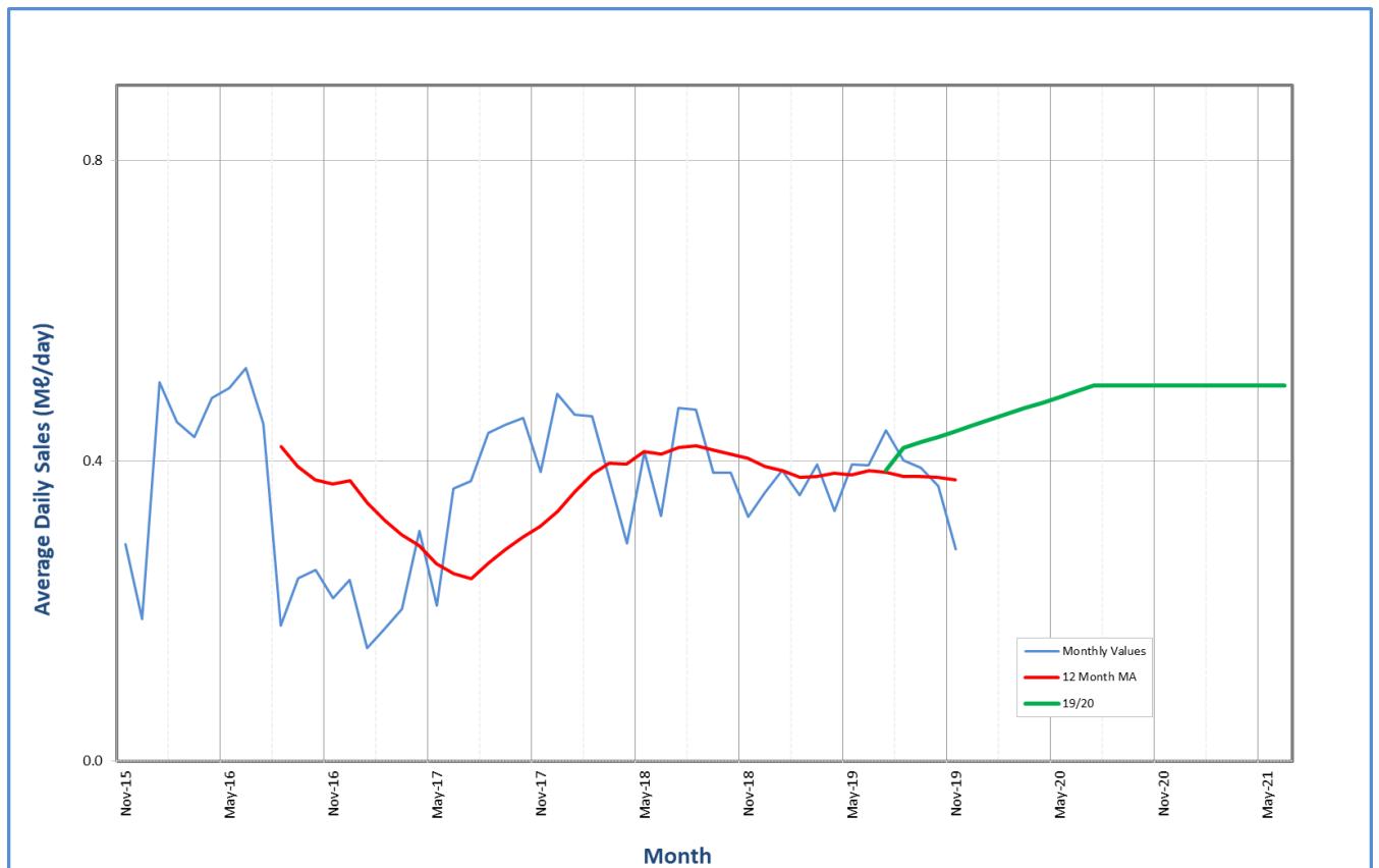
Figure 7.77 Water demand from Appelsbosch WTP.
