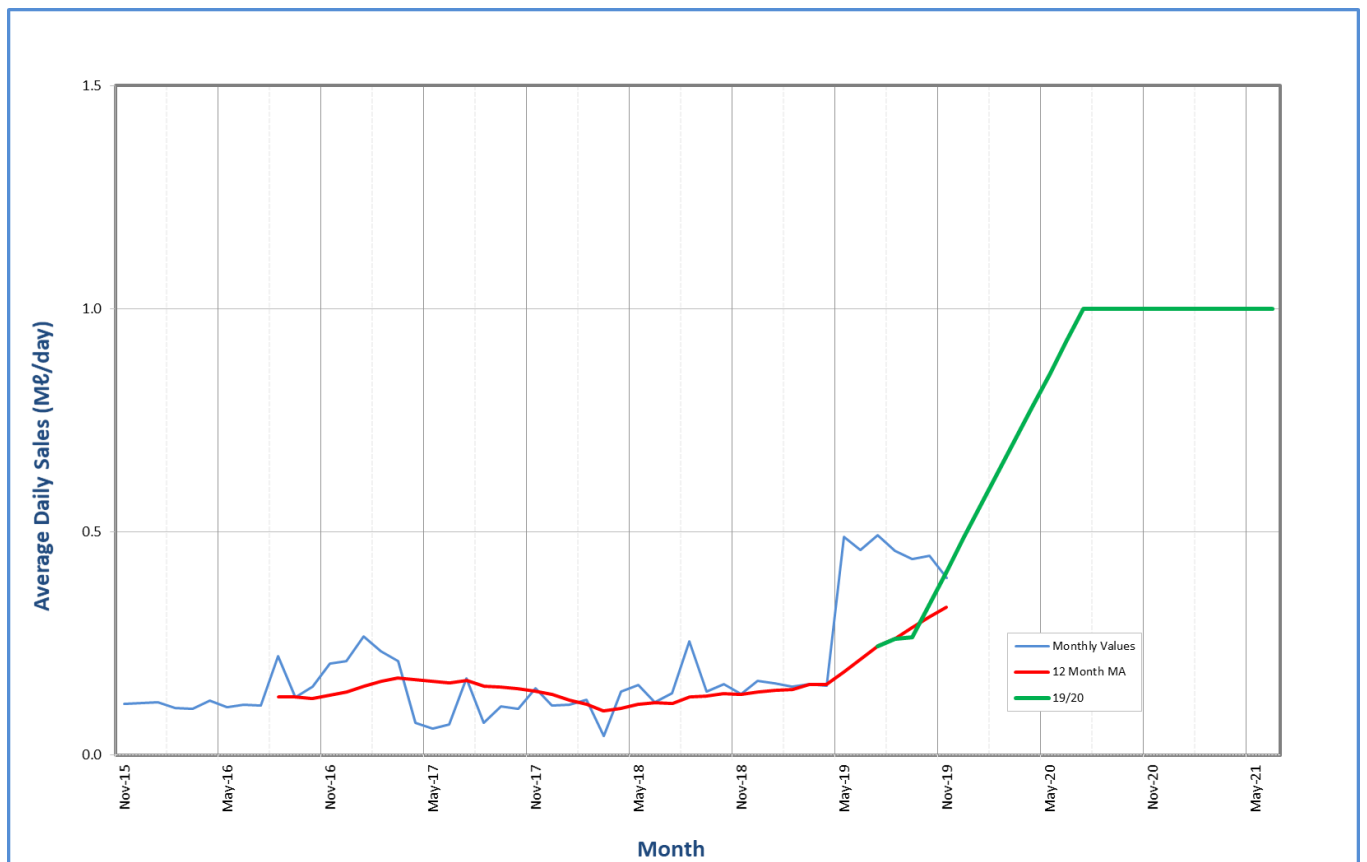
Figure 7.82 Water demand from Lidgetton WTP.
