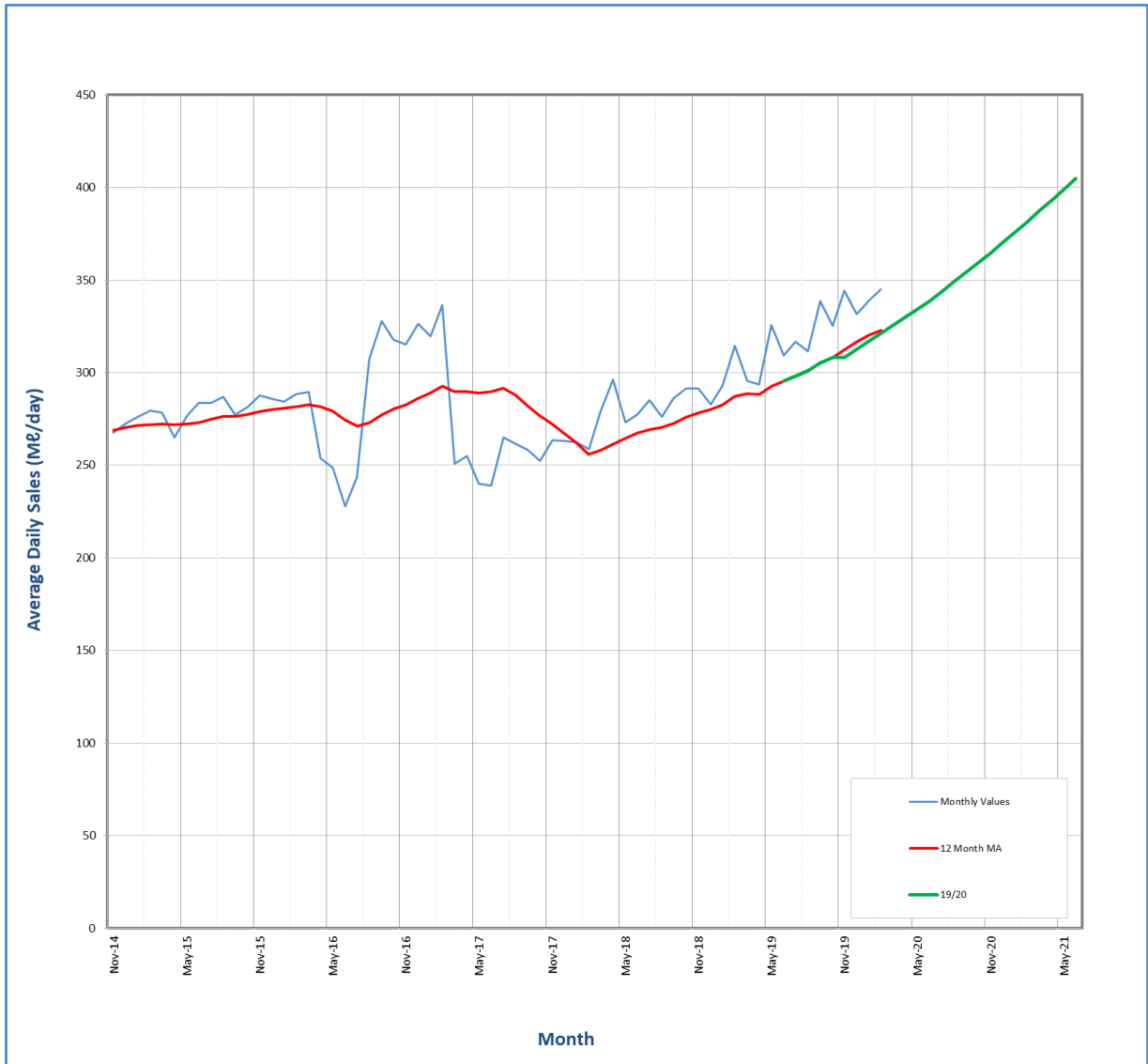
Figure 7.39 Water demand from Midmar WTP.
