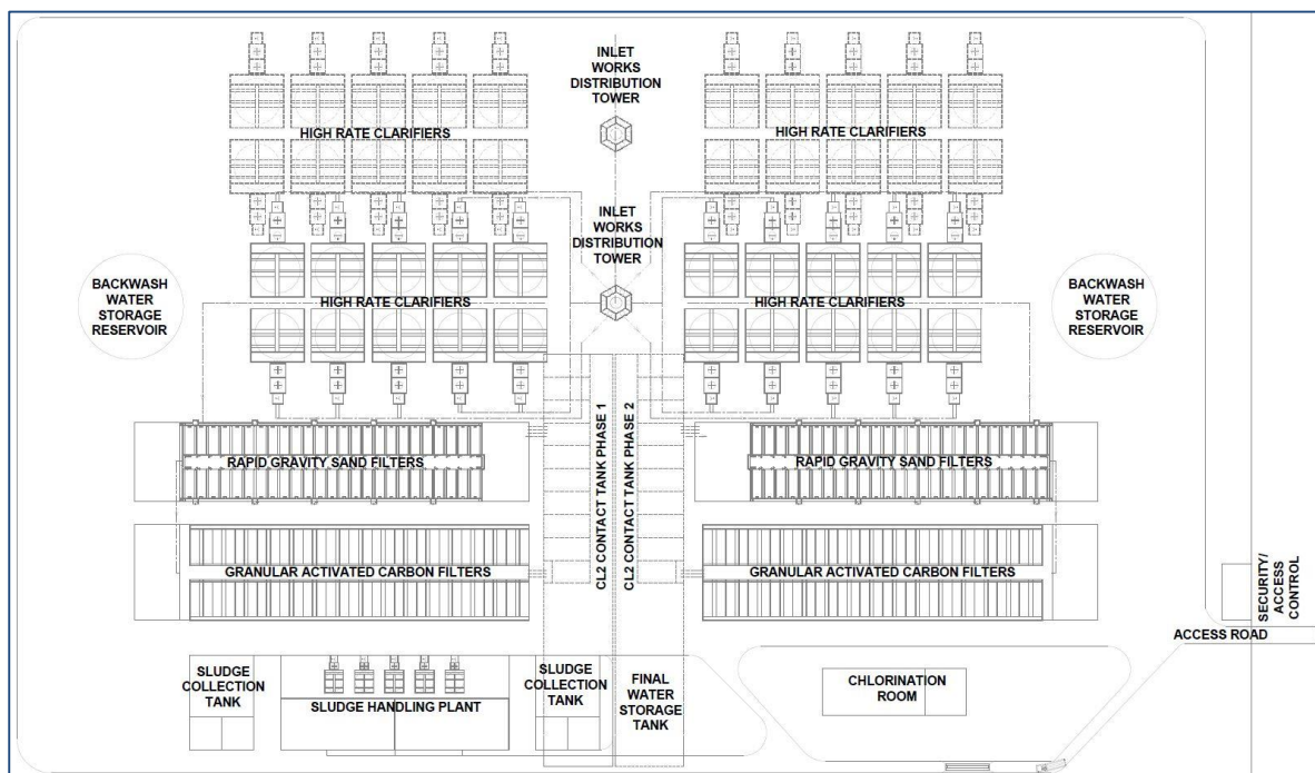
Figure 7.61 Layout of Water Treatment Plant.
