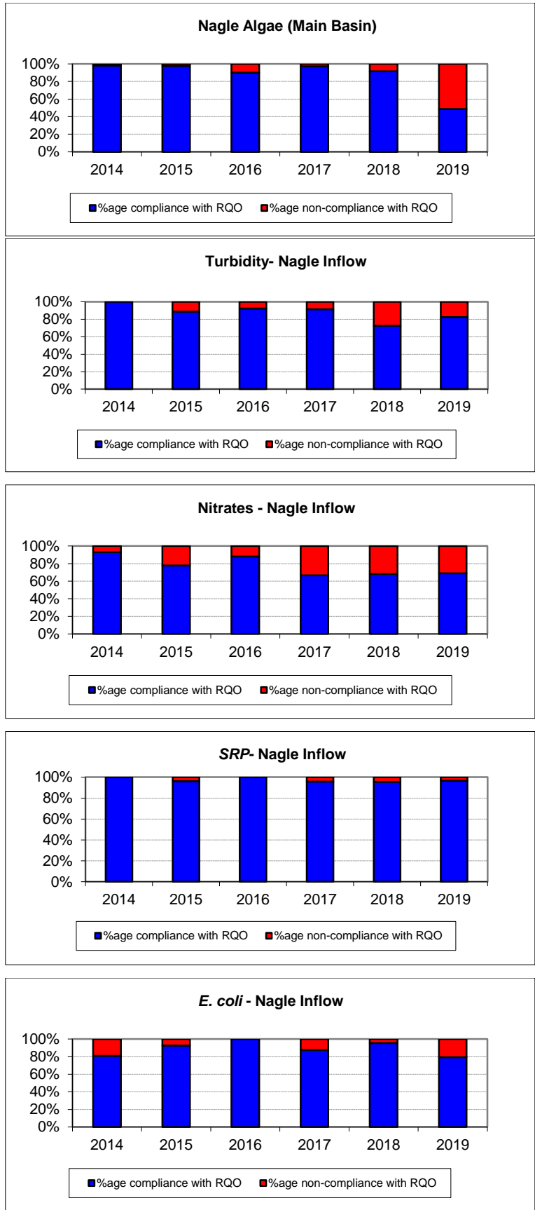
Figure 7.12 Percentage compliance vs. non-compliance with the Resource Quality Objective for Nagle Dam.
