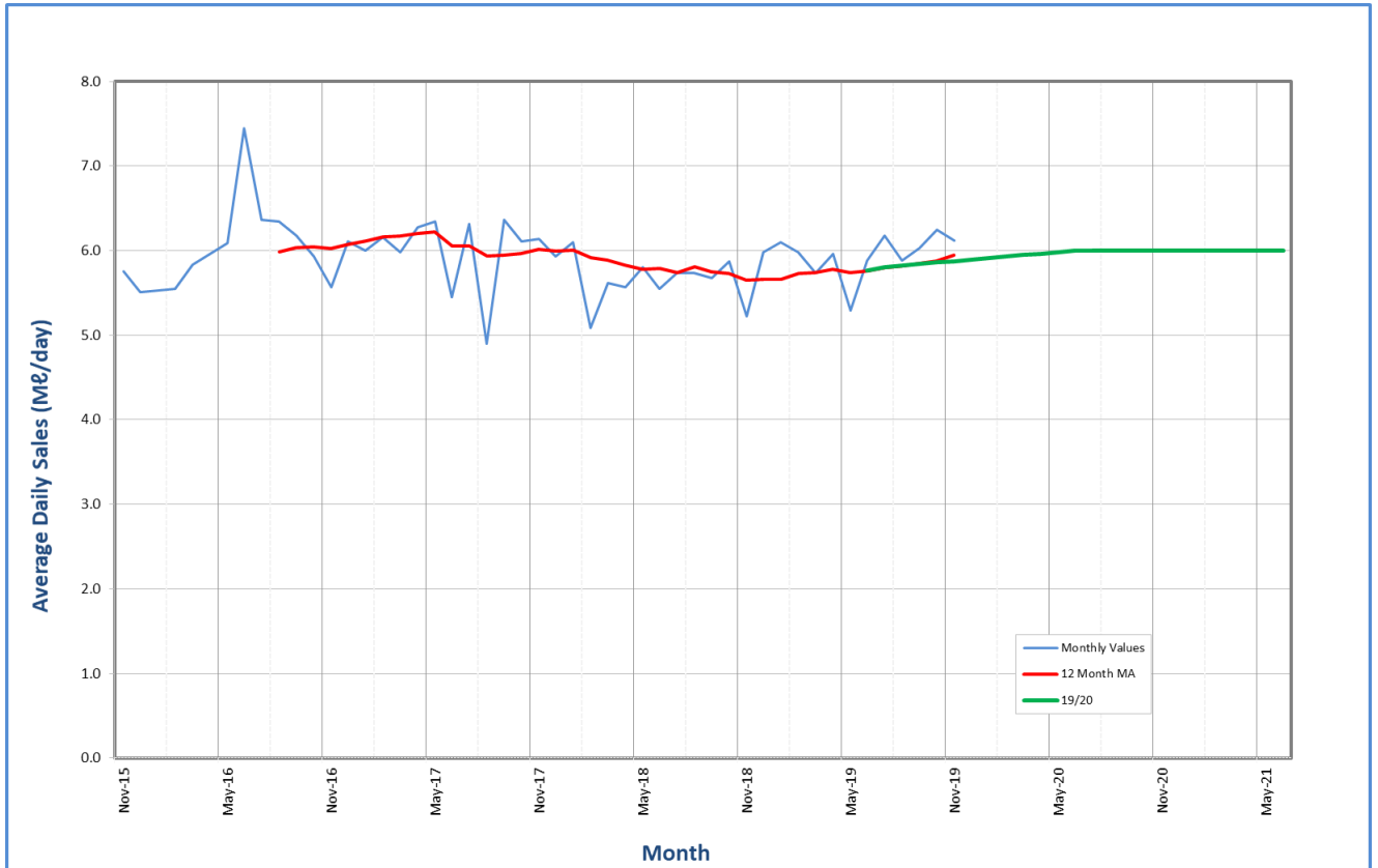
Figure 7.86 Water demand from Mpofana WTP.
