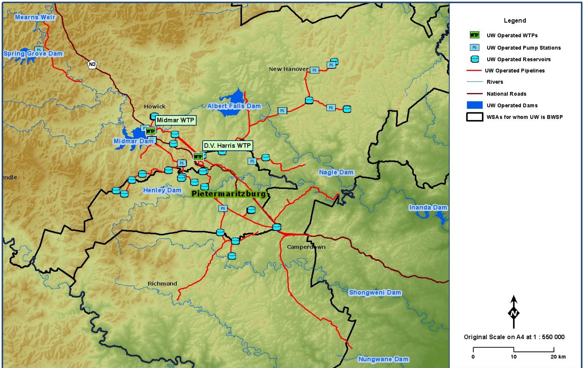
Figure 7.3 General layout of the Upper Mgeni System.
