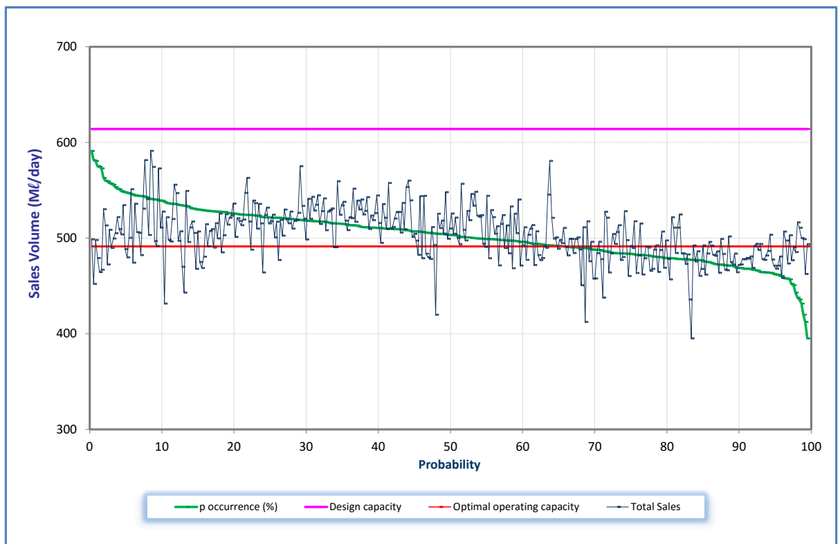
Figure 7.43 Analysis of historical production at Durban Heights WTP from November 2018 to October 2019.
