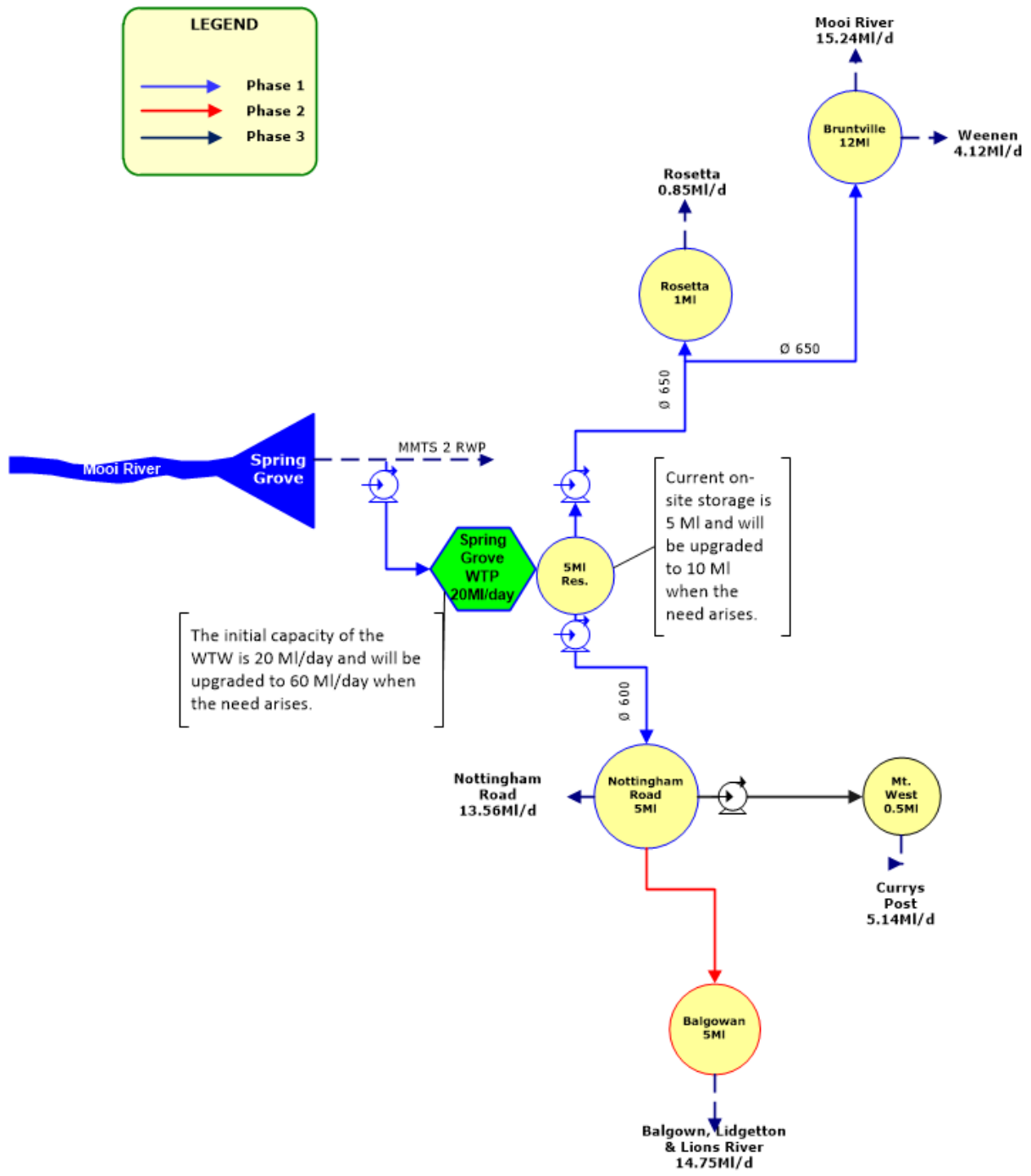
Figure 7.65 Schematic of Greater Mpofana BWSS.
