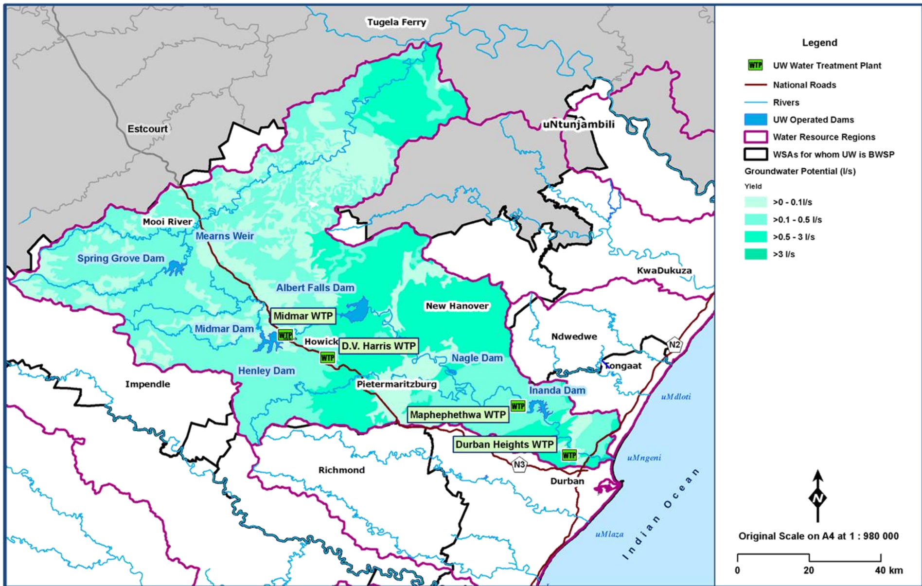
Figure 7.8 Groundwater potential in the Mooi/Mgeni Region (KZN DoT 2011; MDB 2016; Umgeni Water 2017; WR2012).
