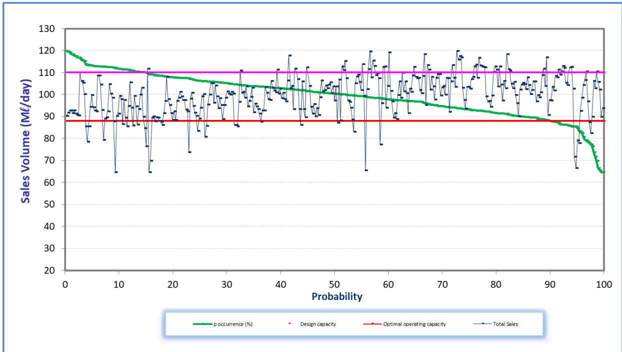
Figure 7.42 Analysis of historical production at D.V. Harris WTP (November 2018 to October 2019).
