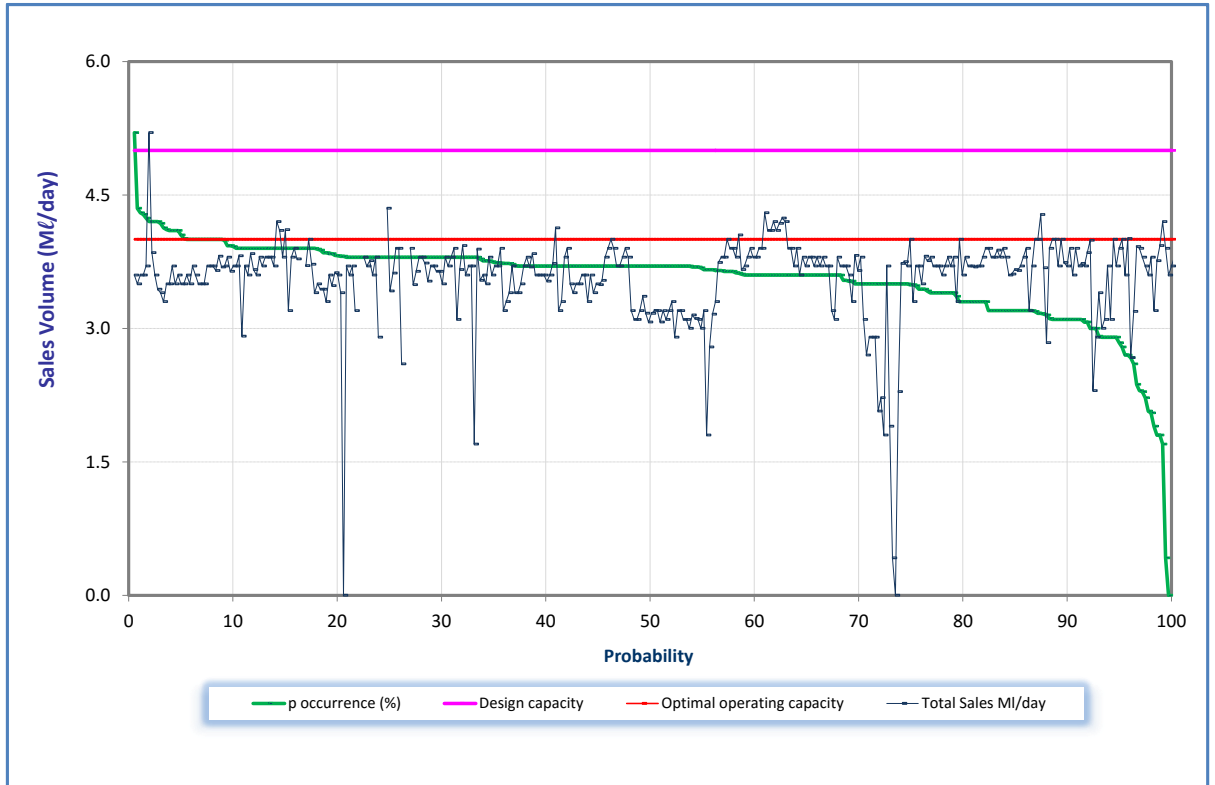
Figure 7.49 Analysis of historical production at Maphephethwa WTP from November 2017 to October 2018.
