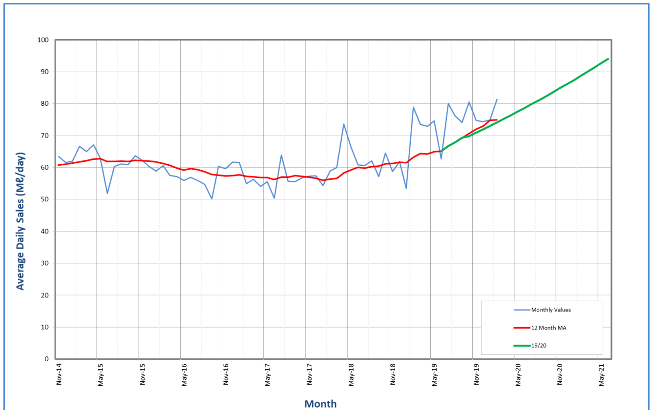
Figure 7.41 Water demand from D. V. Harris WTP.
