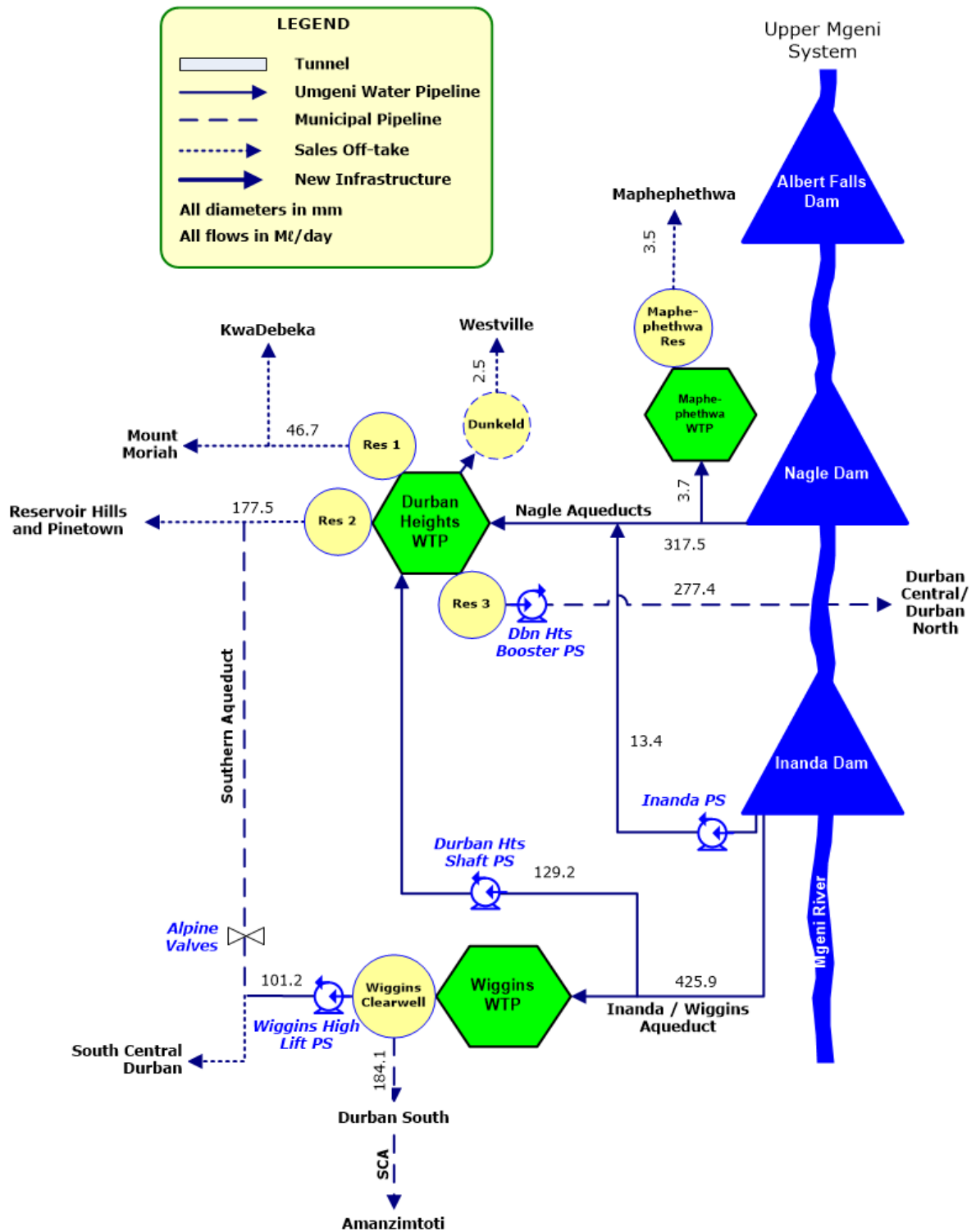
Figure 7.59 Schematic of the Lower Mgeni System.
