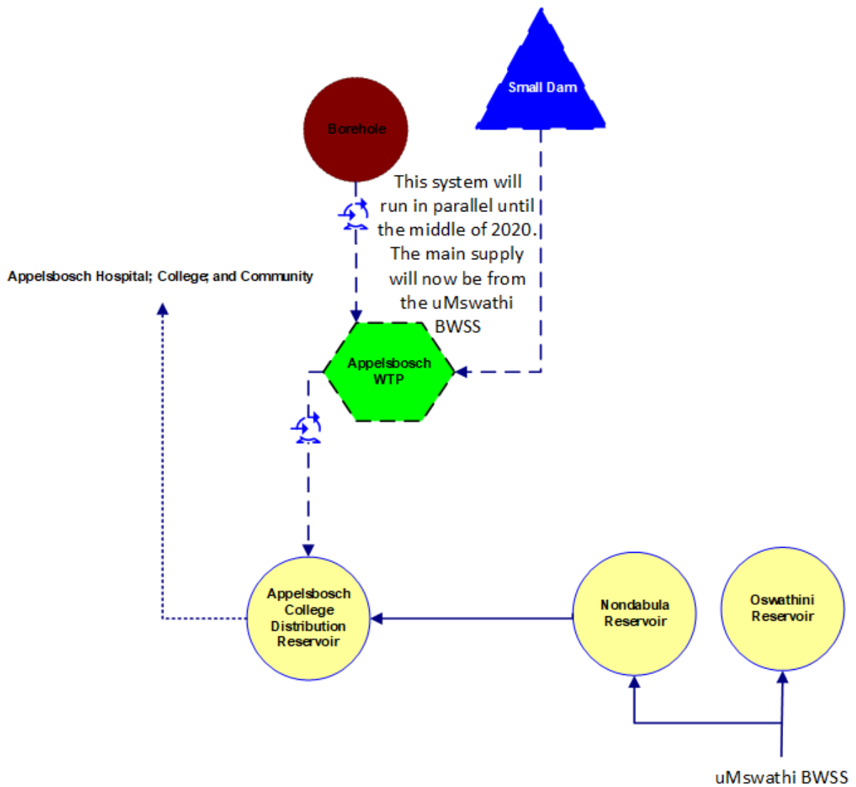
Figure 7.75 Schematic of the Appelsbosch System (subject to verification).
