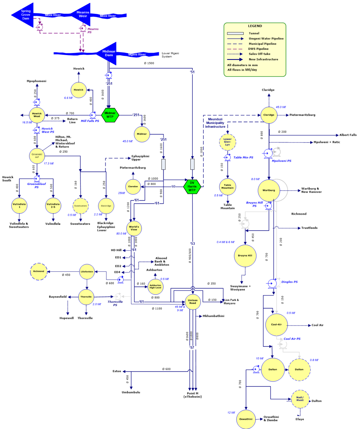
Figure 7.4 Schematic of the Upper Mgeni System.
