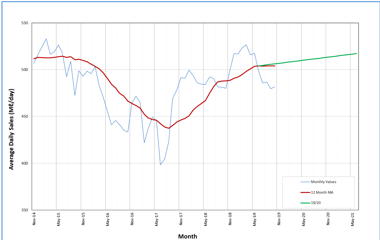
Figure 7.44 Historical demand curve for Durban Heights WTP.
