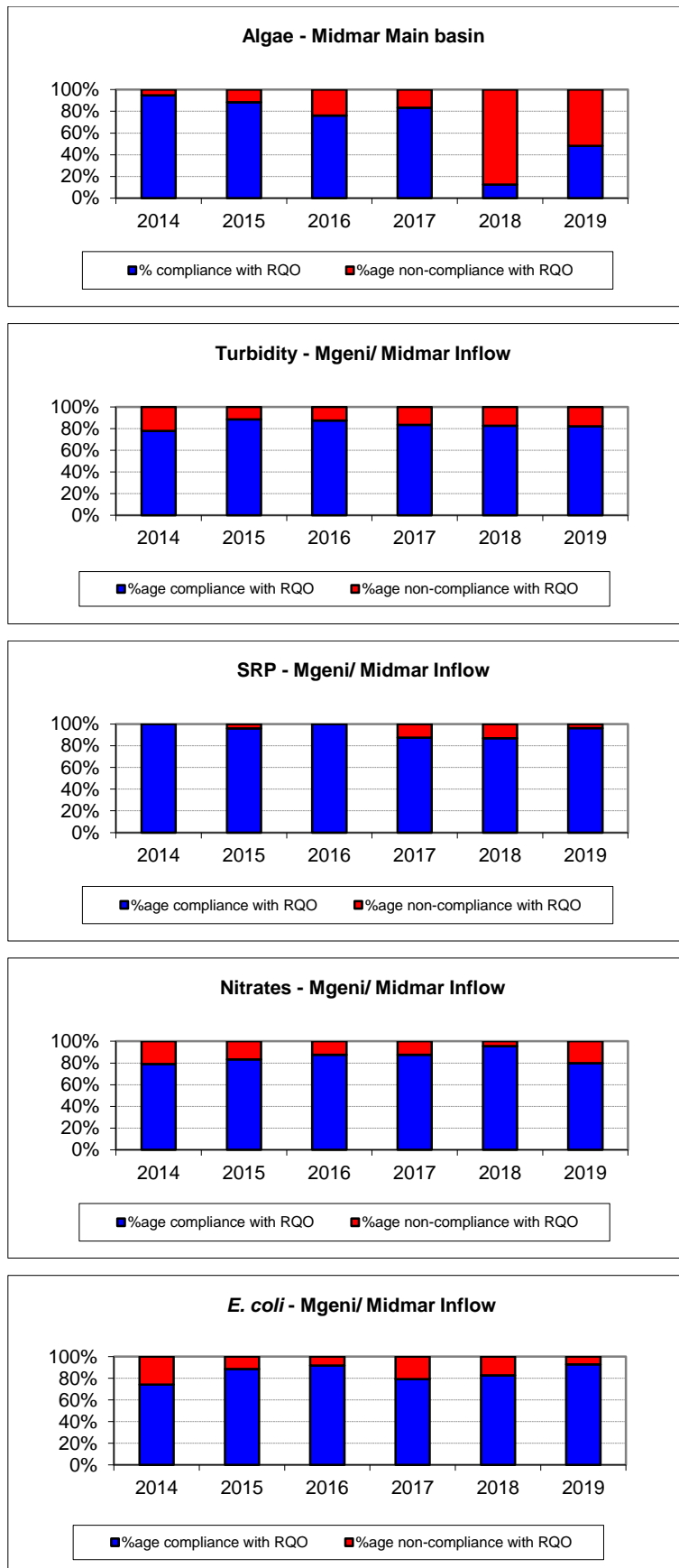
Figure 7.9 Percentage compliance vs. non-compliance with the Resource Quality Objective for Midmar Dam.
