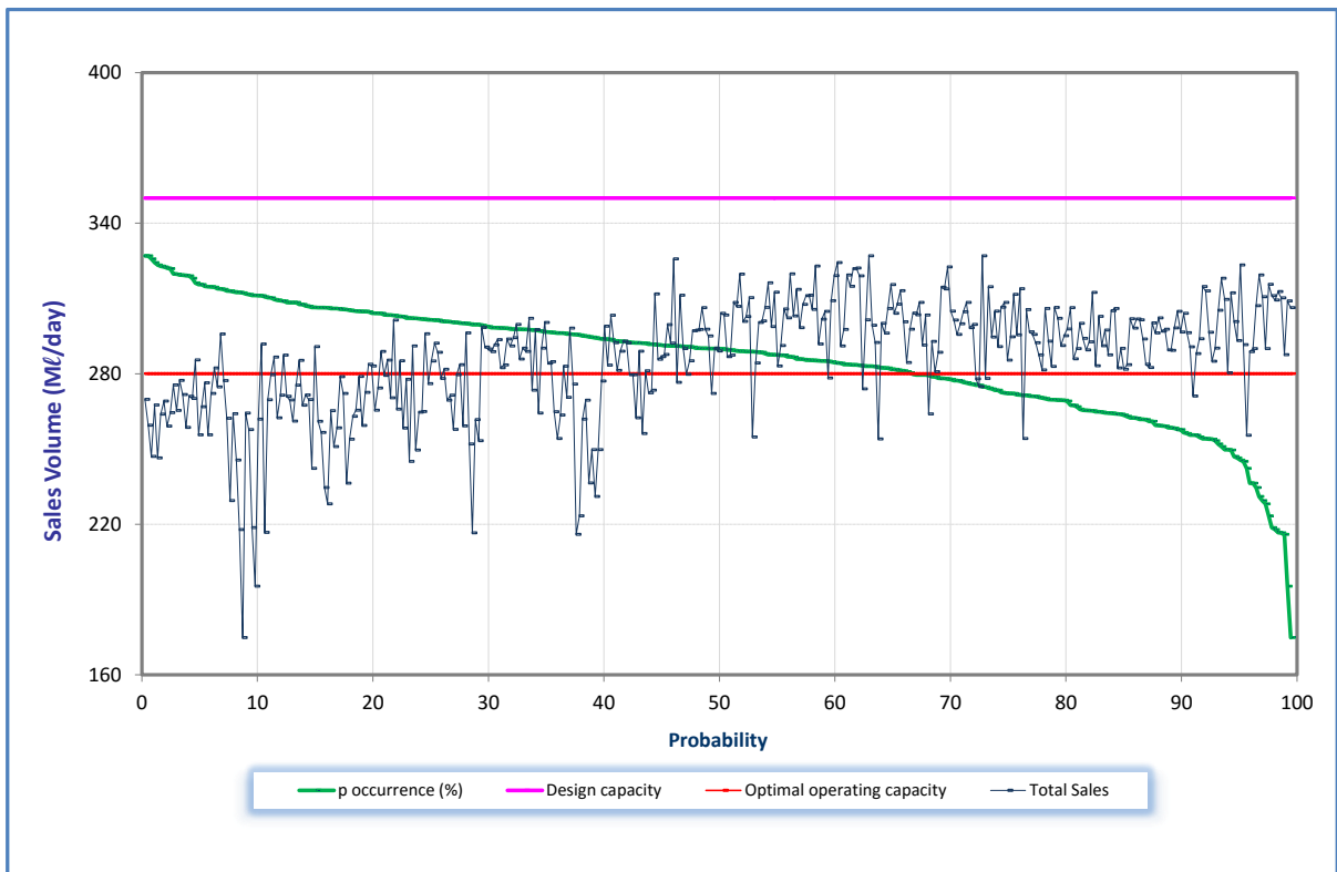
Figure 7.46 Analysis of historical production at Wiggins WTP from November 2017 to October 2018.
