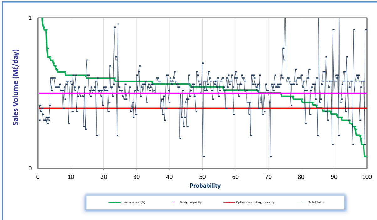
Figure 7.90 Analysis of historical production at Rosetta WTP (November 2018 to October 2019).
