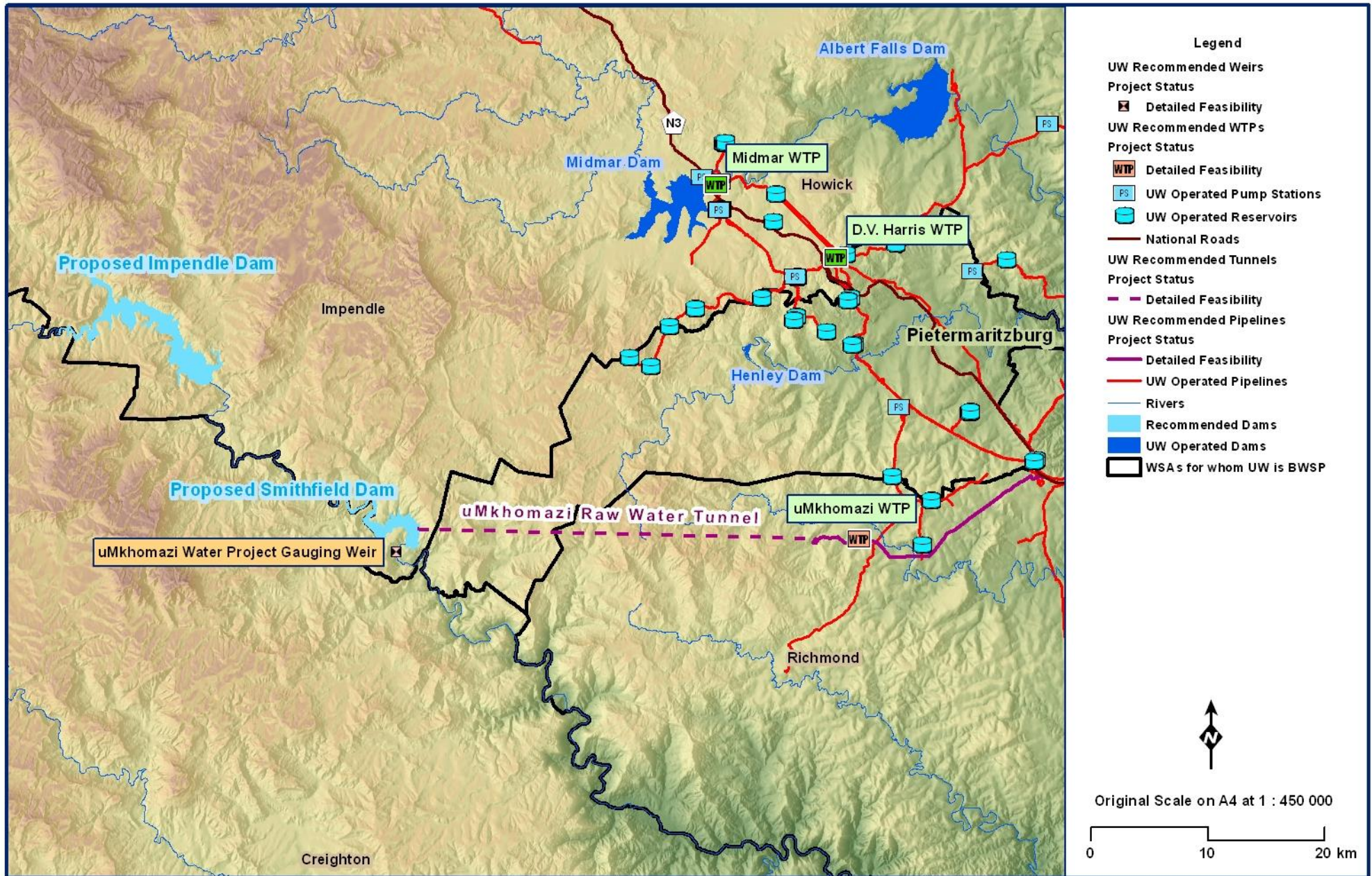
Figure 7.60 uMkhomazi Water Project.
