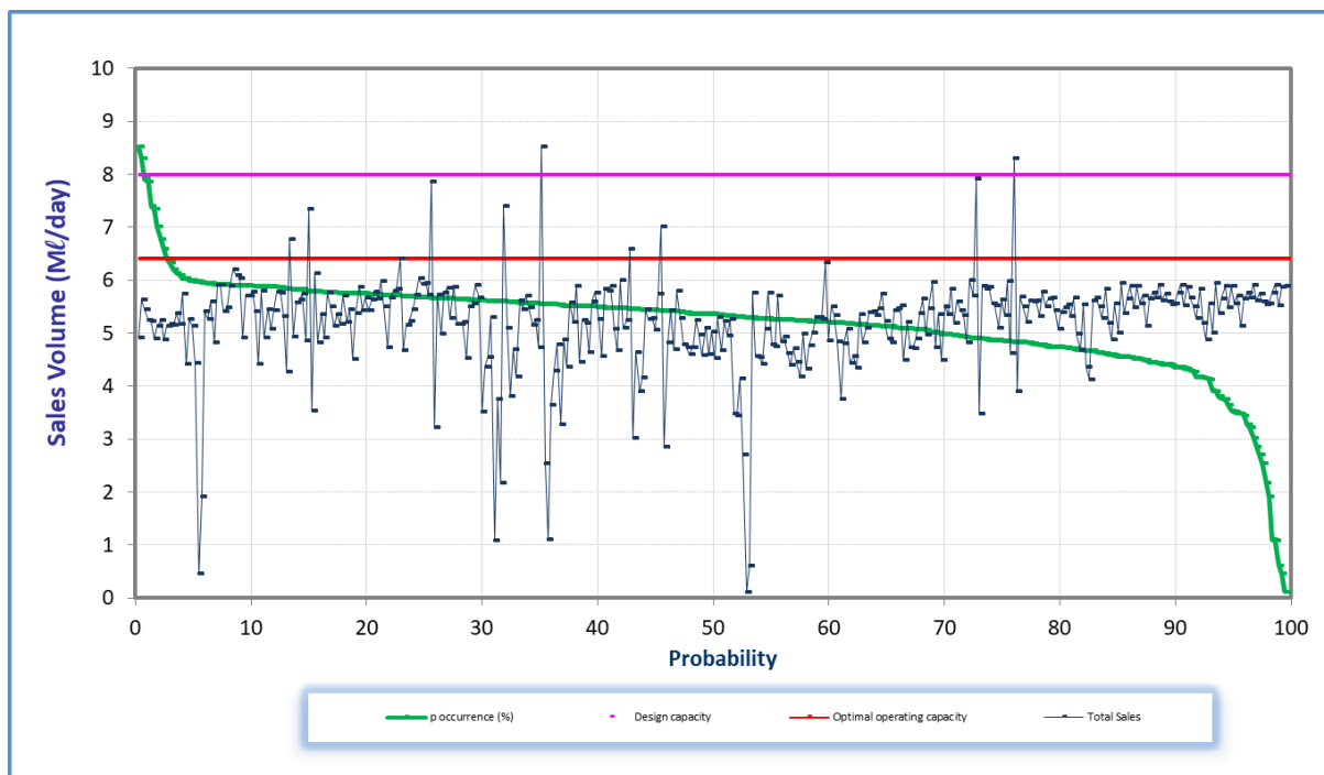
Figure 7.85 Analysis of historical production at Mpofana WTP (November 2018 to October 2019).
