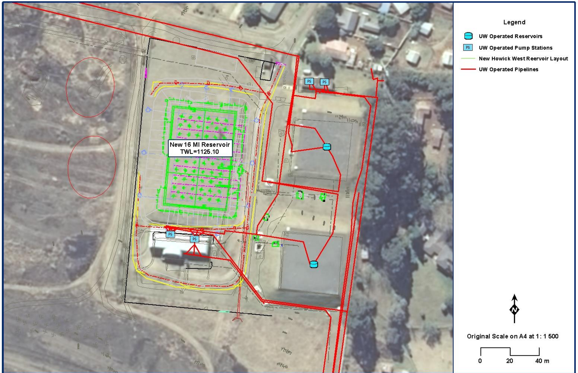
Figure 7.67 General layout of the proposed Howick-West Reservoir.
