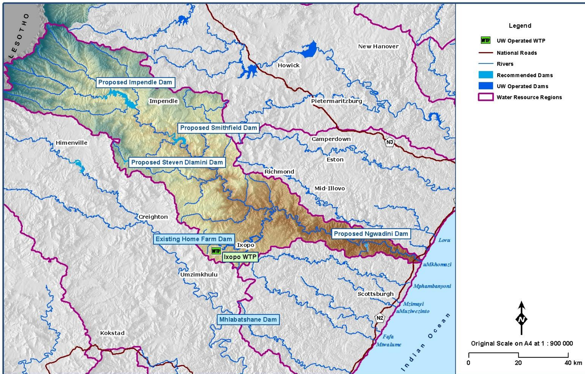
Figure 7.52 Proposed water resource infrastructure in the Mkhomazi Region (KZN DoT 2011; MDB 2016; Umgeni Water 2017; WR2012).
