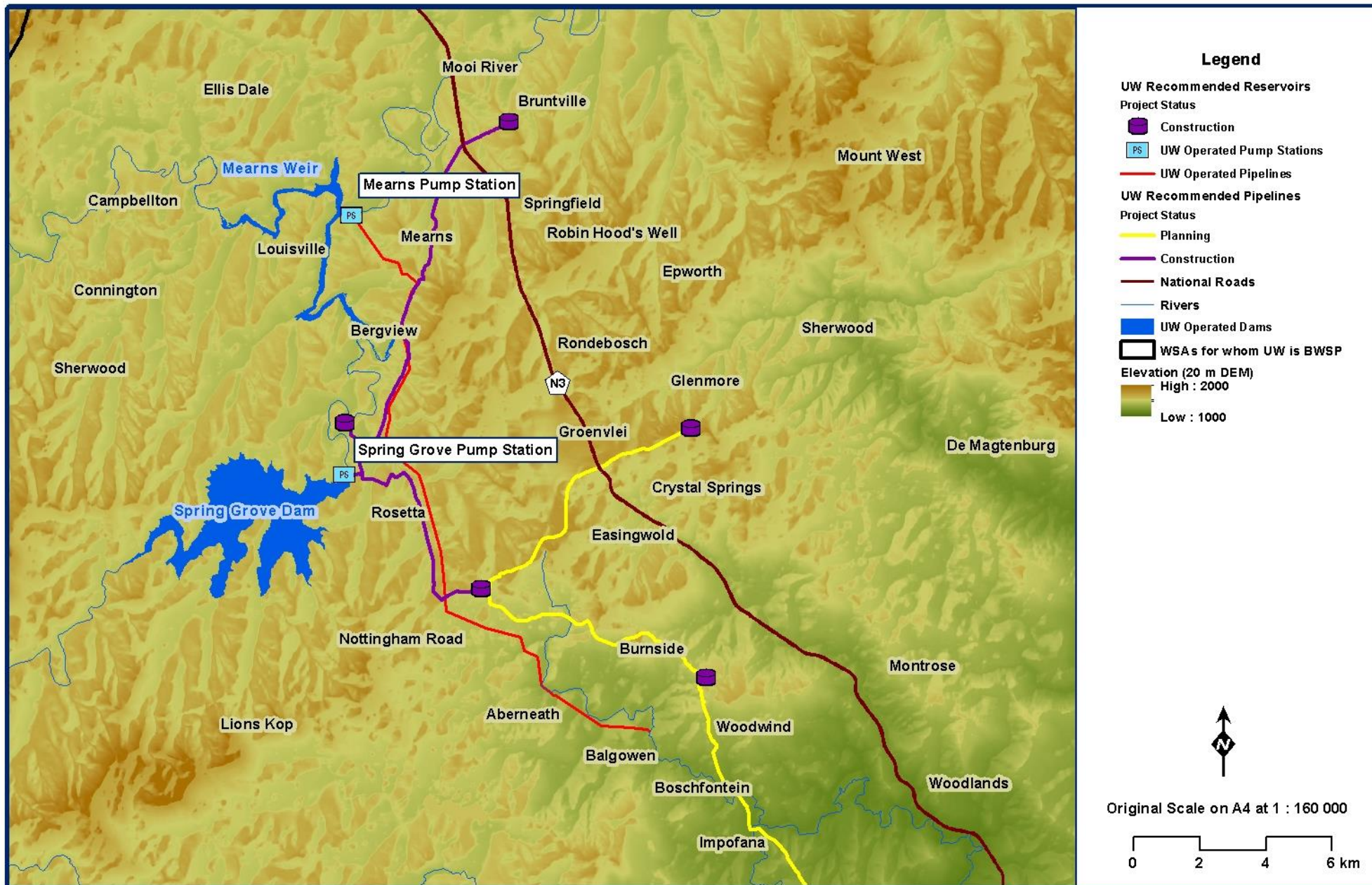
Figure 7.64 Greater Mpozana Bulk Water Supply Scheme.
