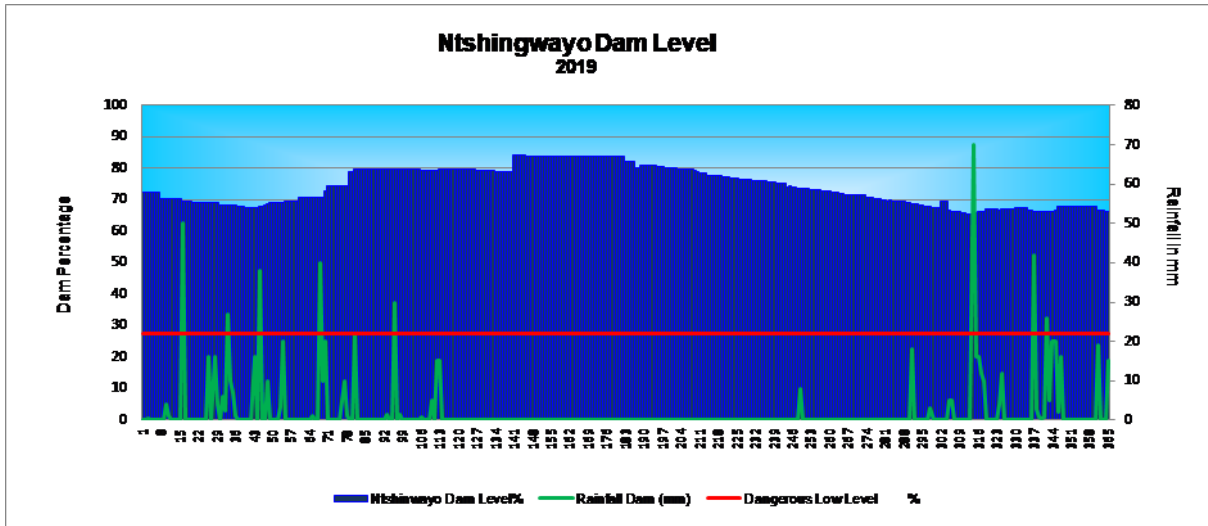
Figure 14.49 Ntshingwayo Dam Level and rainfall figures from July 2019 to June 2020 (uThukela Water 2021)
