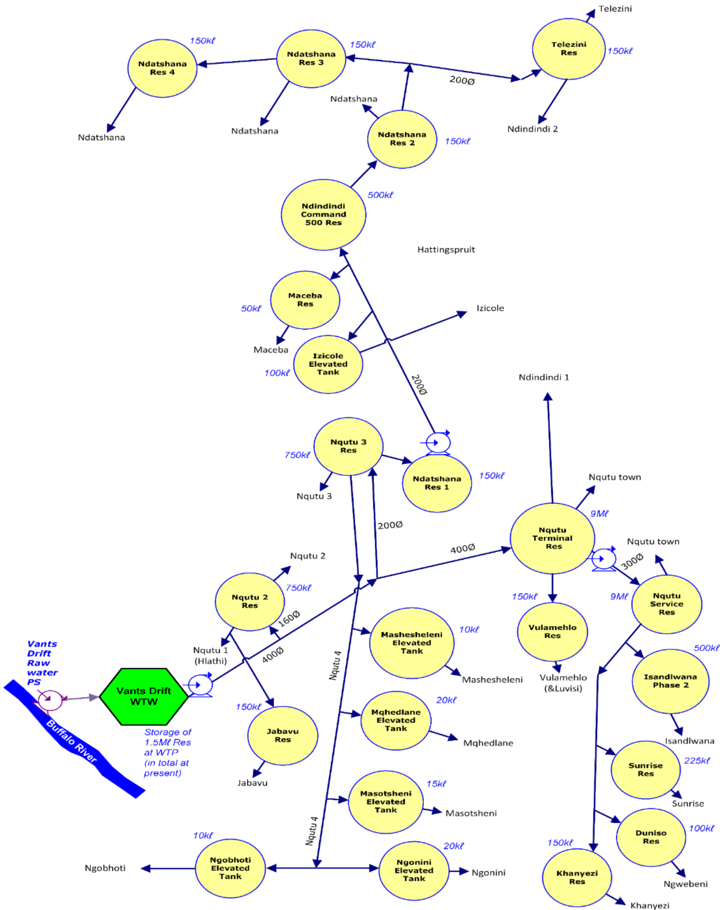
Figure 14.30 Vants Drift WTP Supply Schematic (not to scale; uMzinyathi DM infrastructure)
