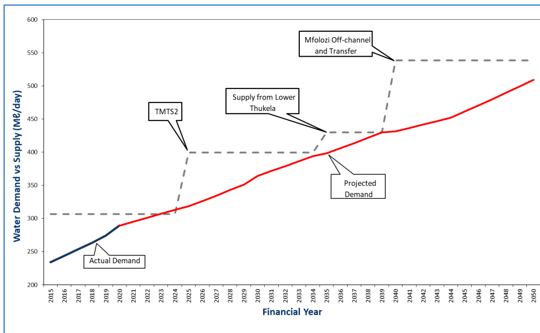
Figure 16.31 uMhlathuze System Balance
