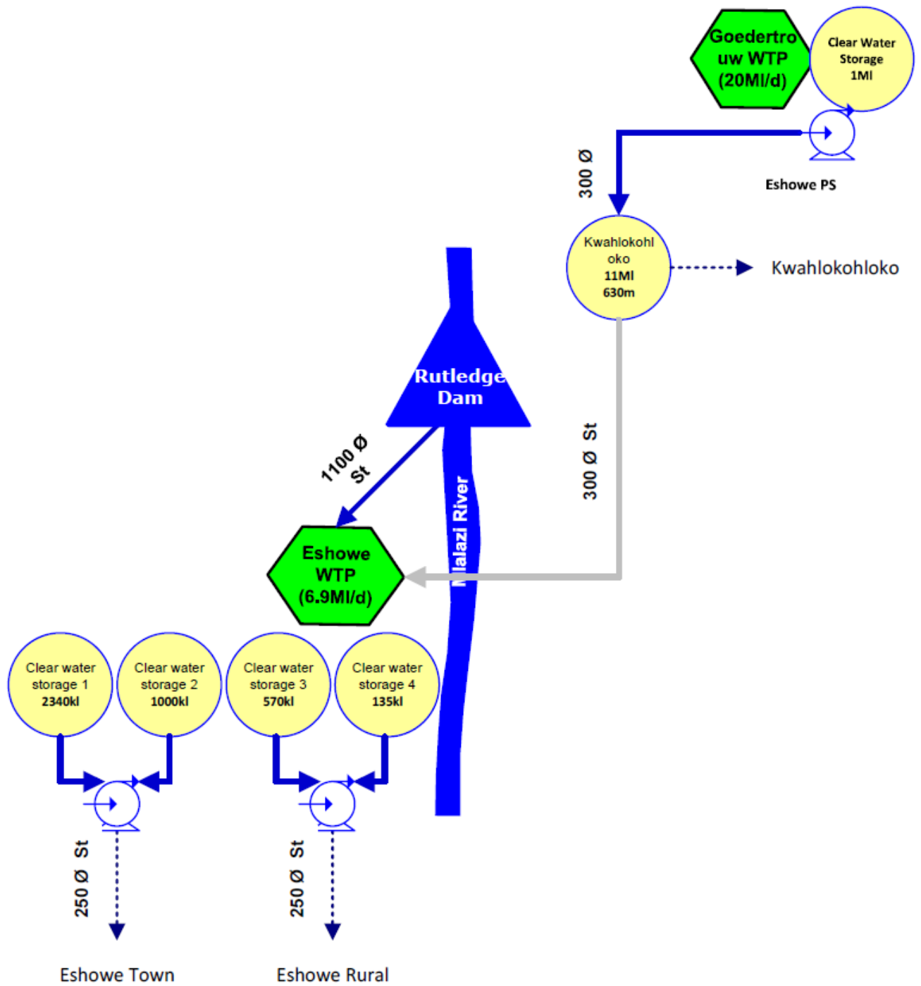
Figure 16.20 Schematic of Eshowe System.
