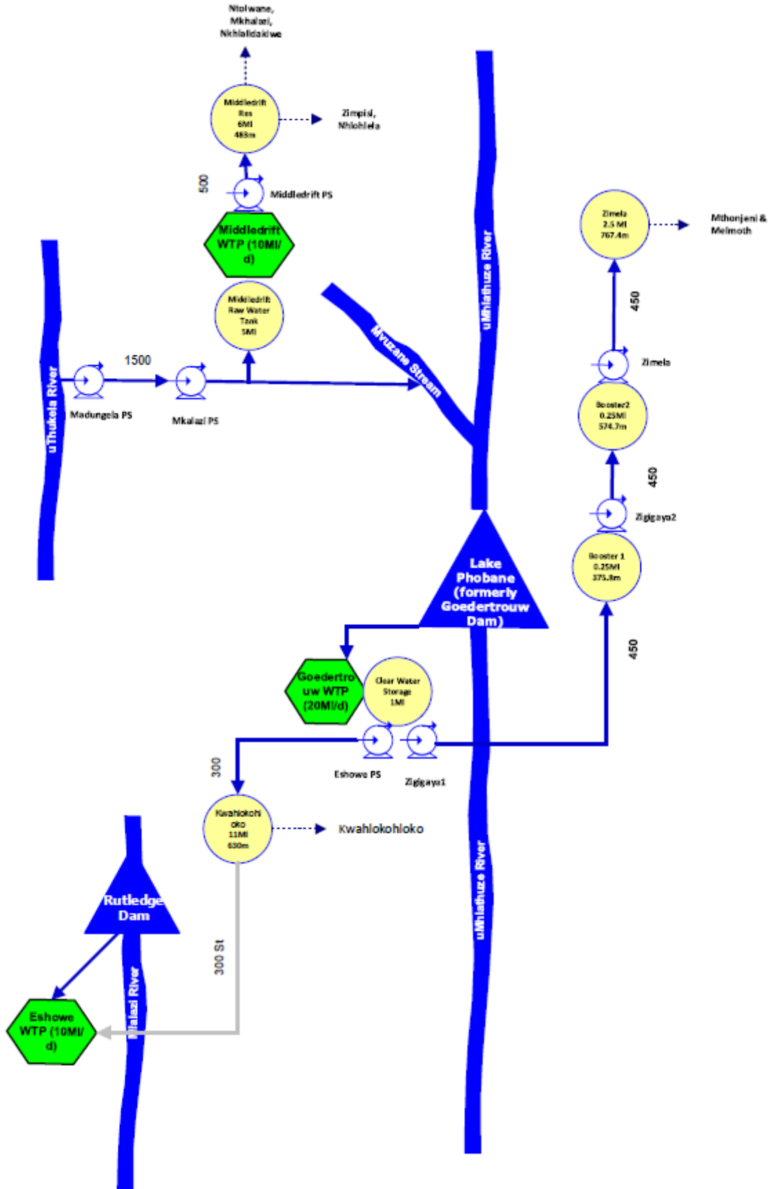
Figure 16.16 Schematic of Central uMhlathuze System
