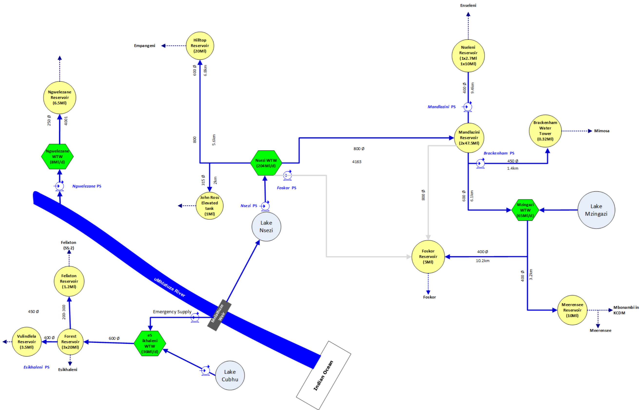
Figure 16.22 Schematic of CoU System
