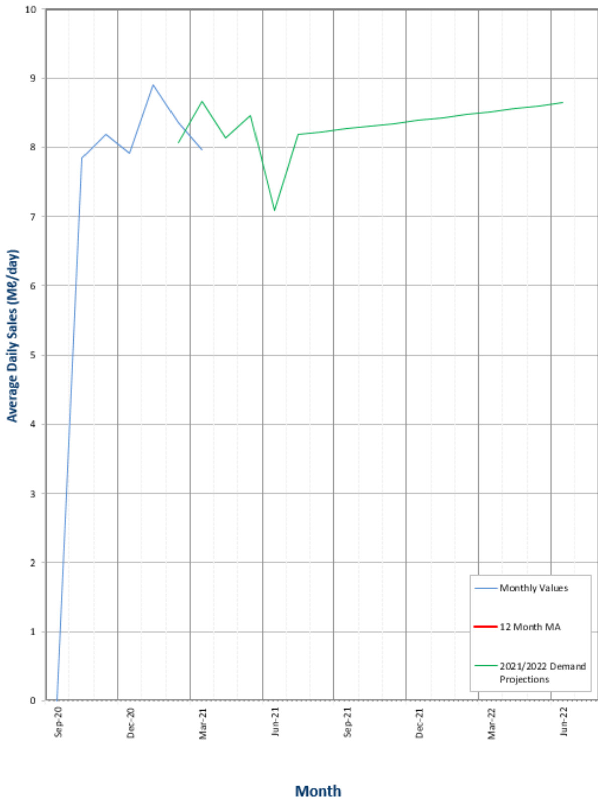
Figure 16.28 Water demand for Middledrift WTP
