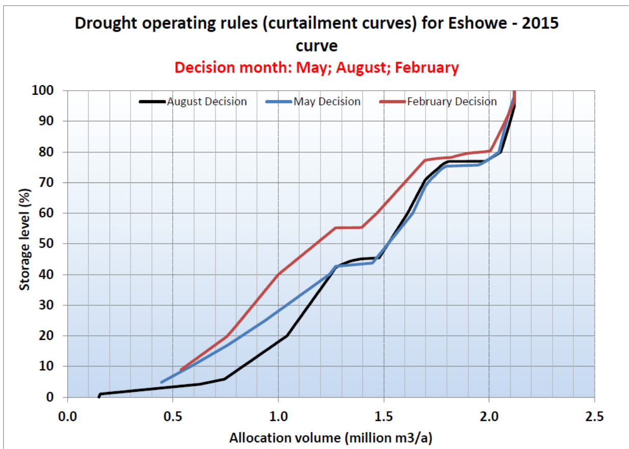
Figure 16.7 Drought Operating Rules (Curtailment curves) for Eshowe (DWS 2015:6-9)
