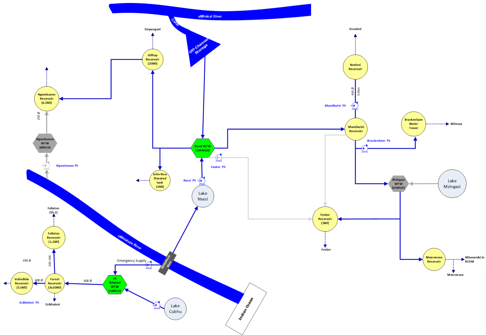
Figure 16.32 Future Bulk Scenario for CoU
